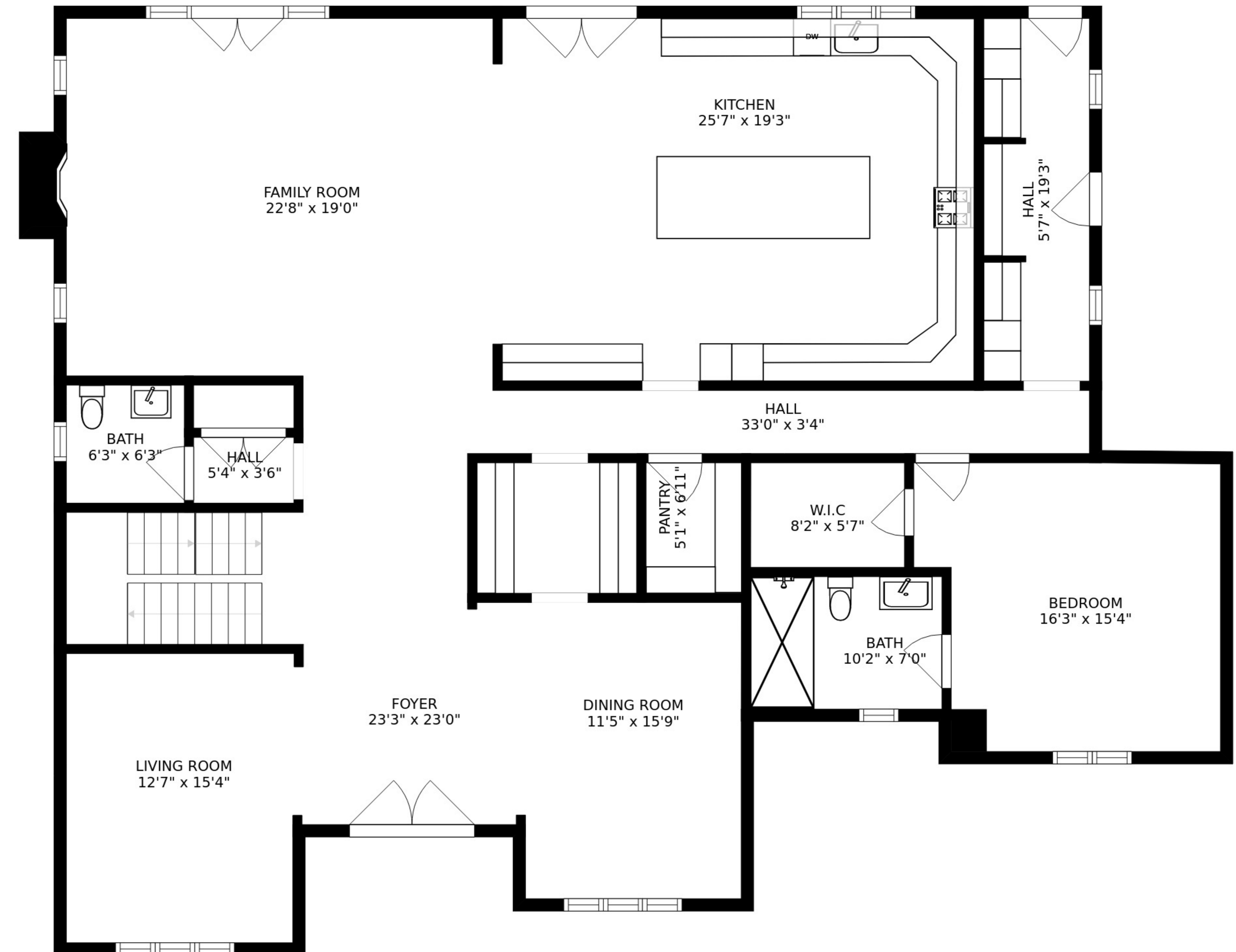
FLOOR 2
