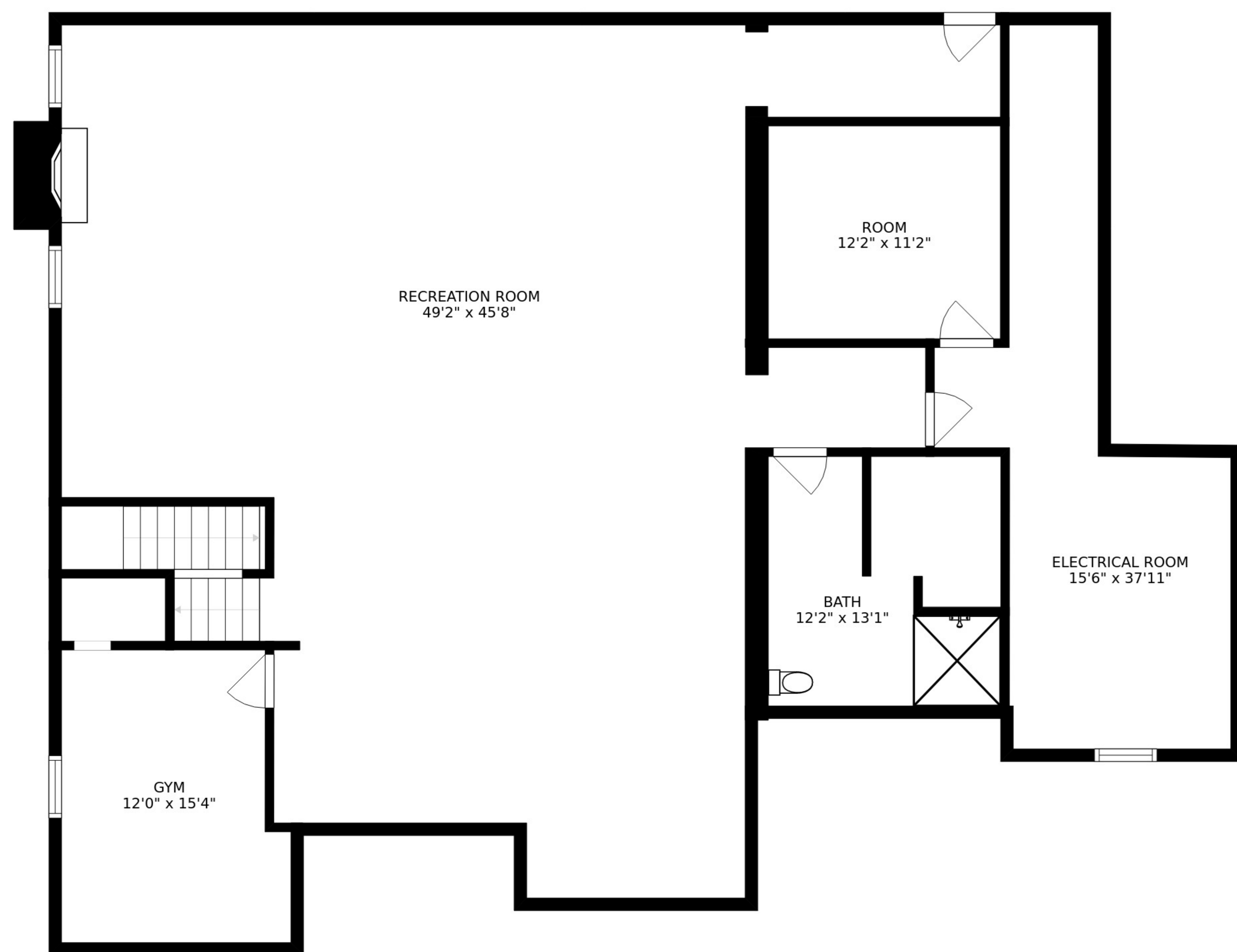
FLOOR 1
