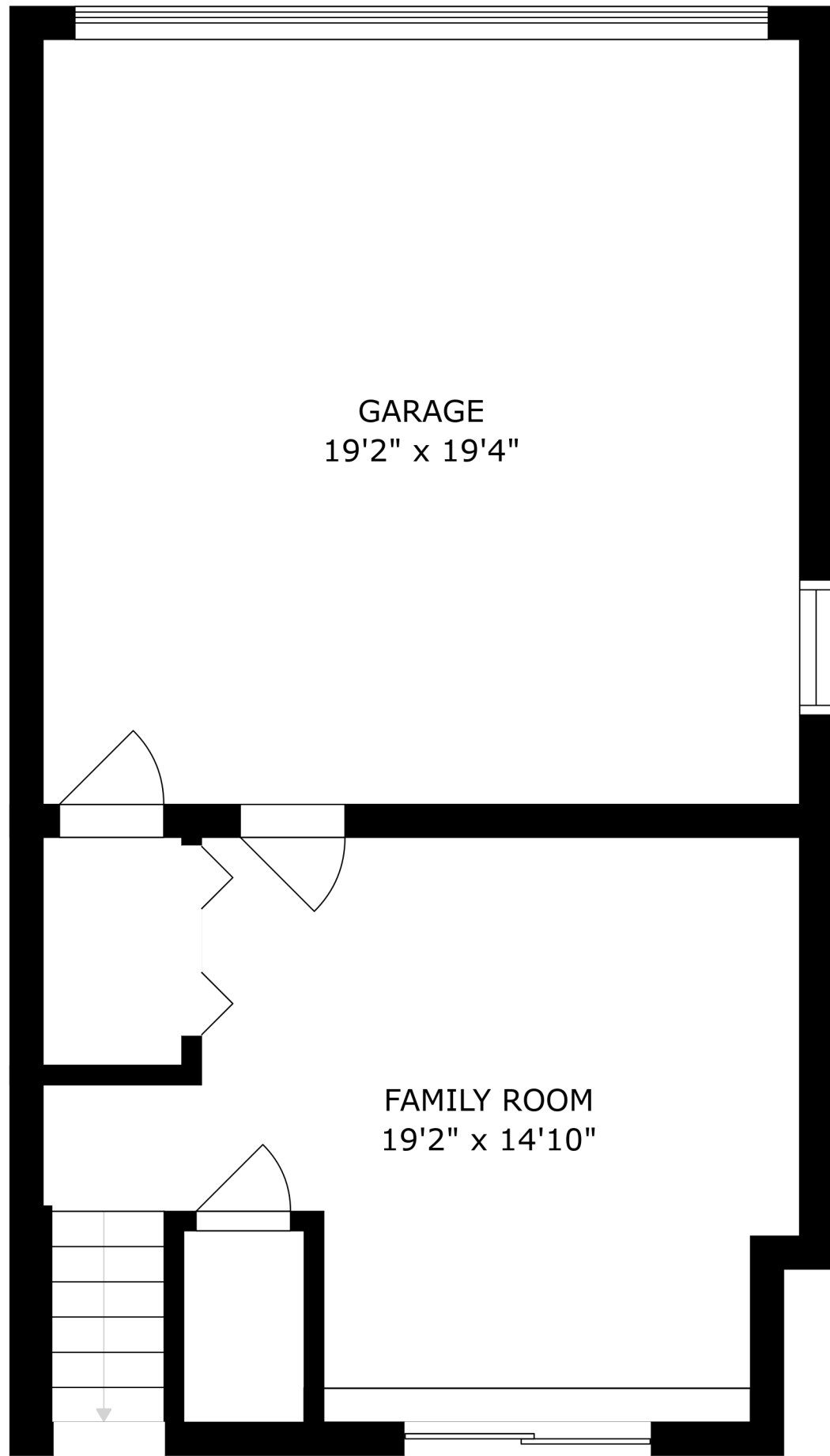
WALKOUT BASEMENT
