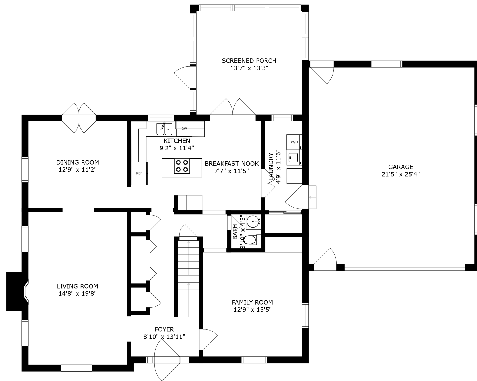
FLOOR 2
