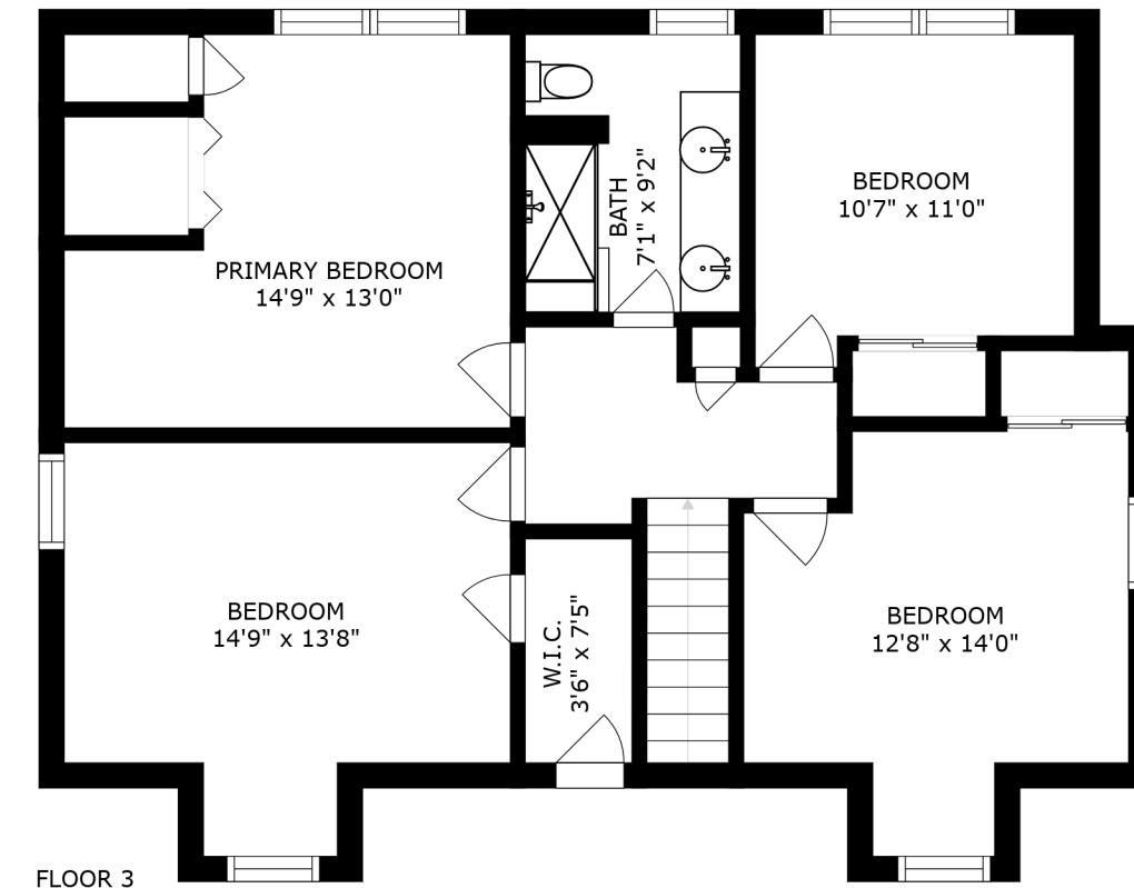
FLOOR 3
