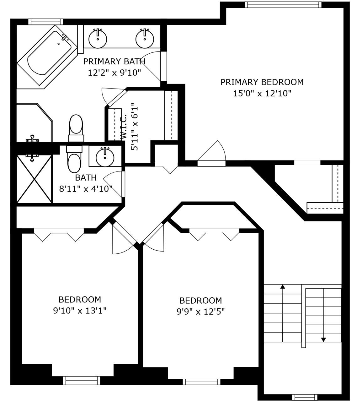
FLOOR 3
