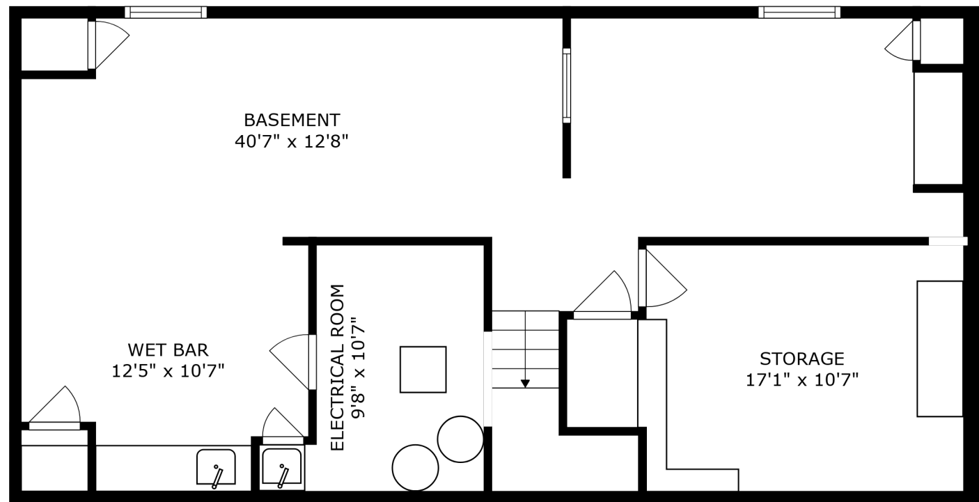
FLOOR 1
