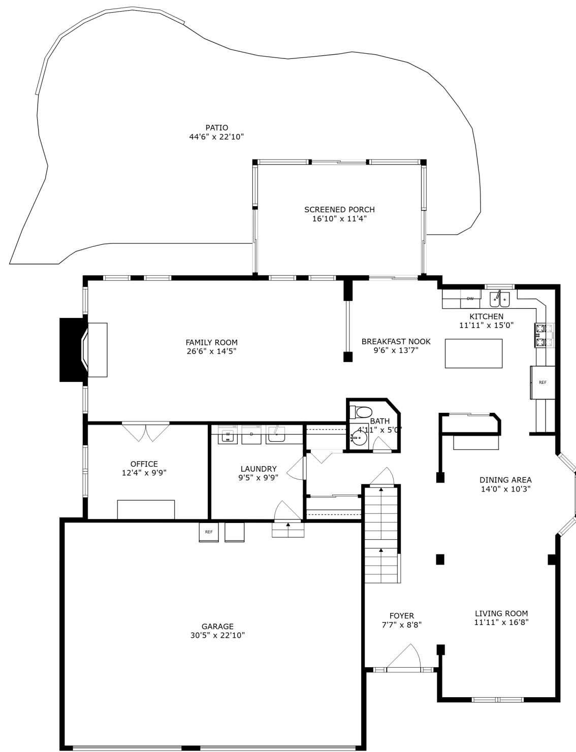
FLOOR 2
