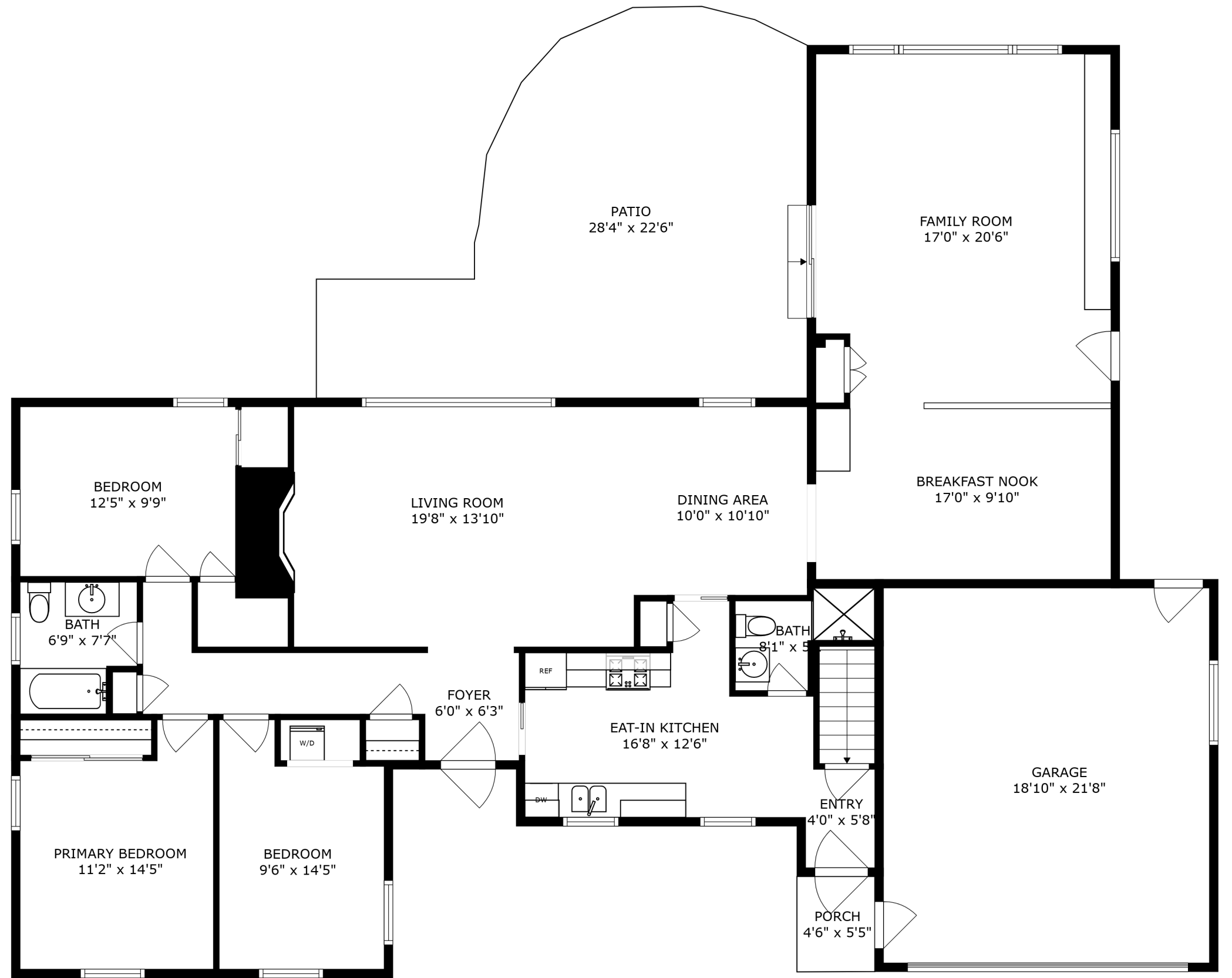
FLOOR 2
