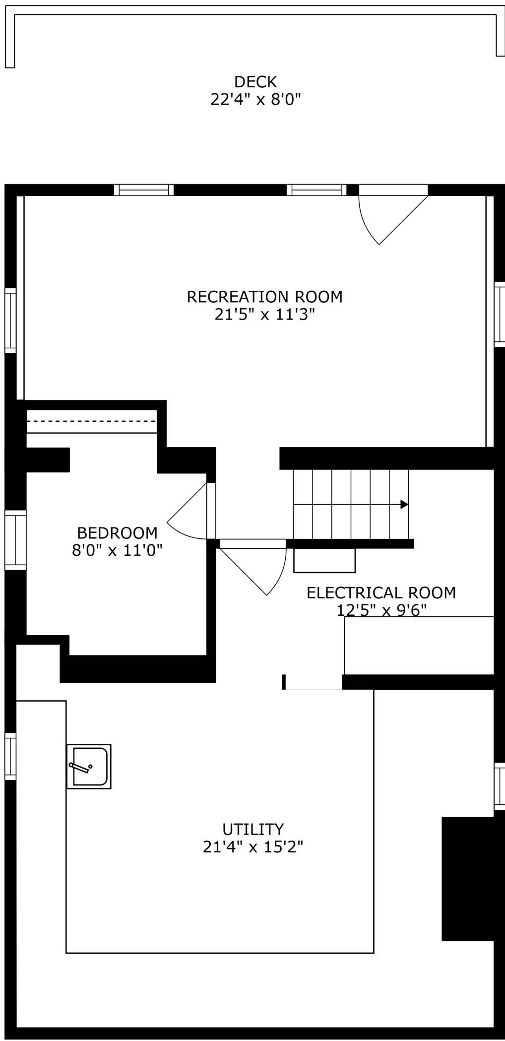
FLOOR 1
