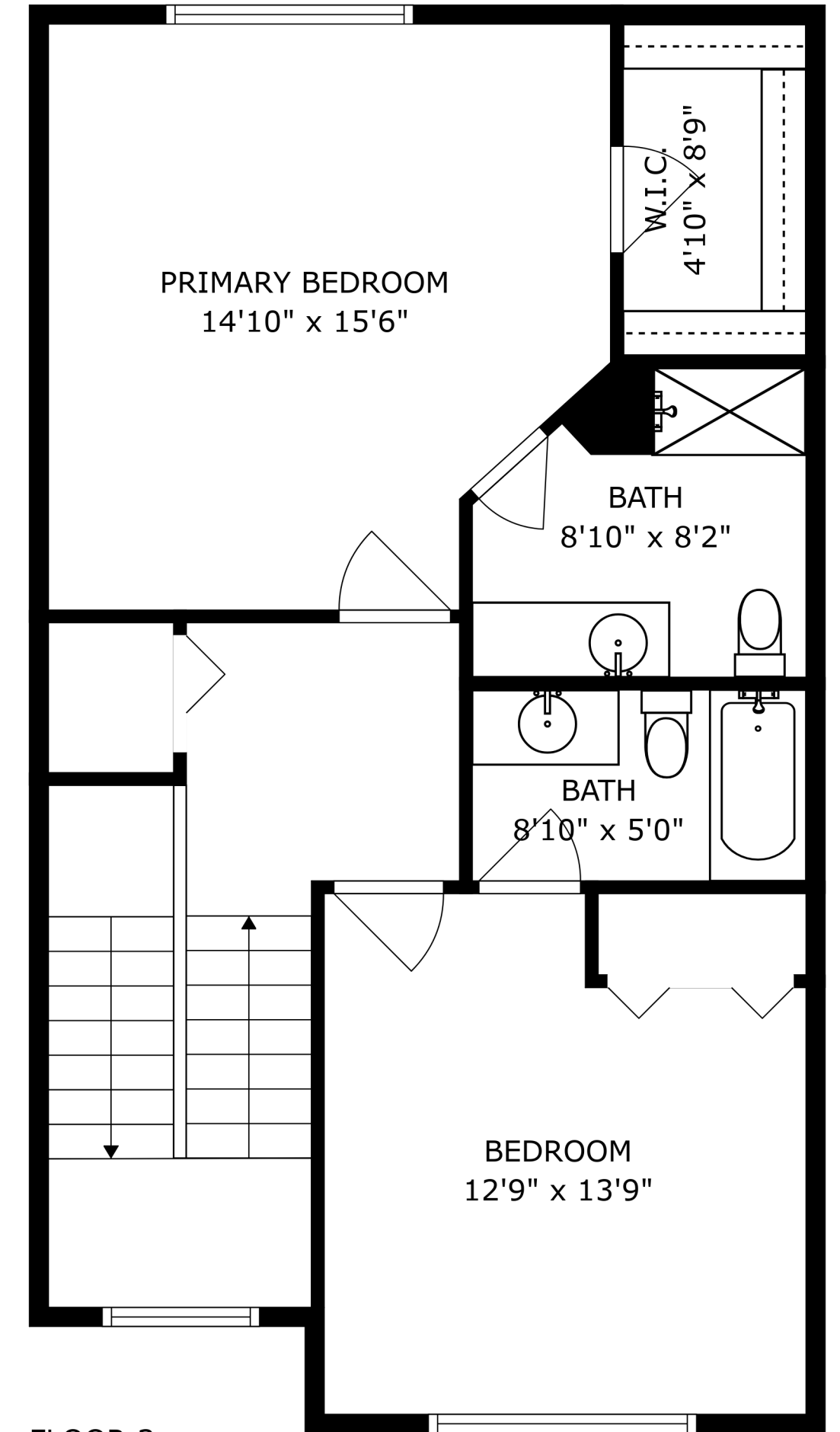
FLOOR 3
