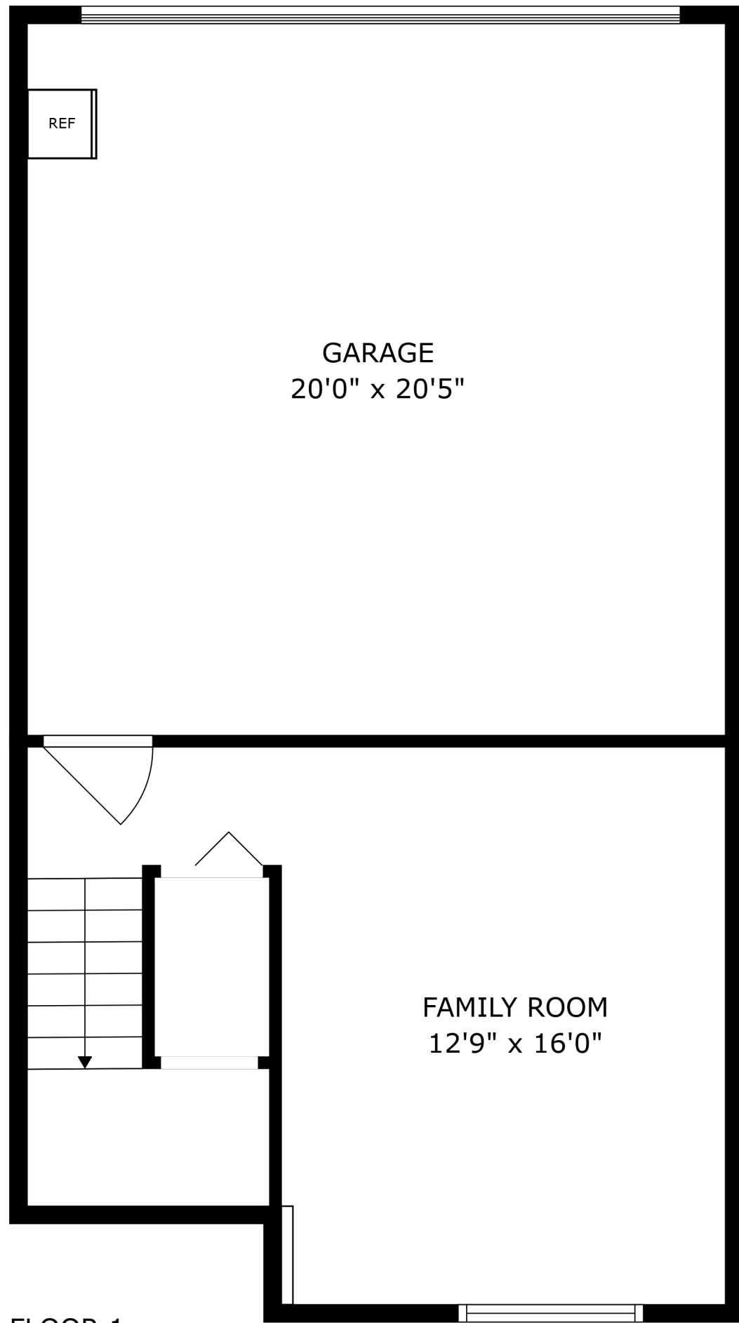
FLOOR 1
