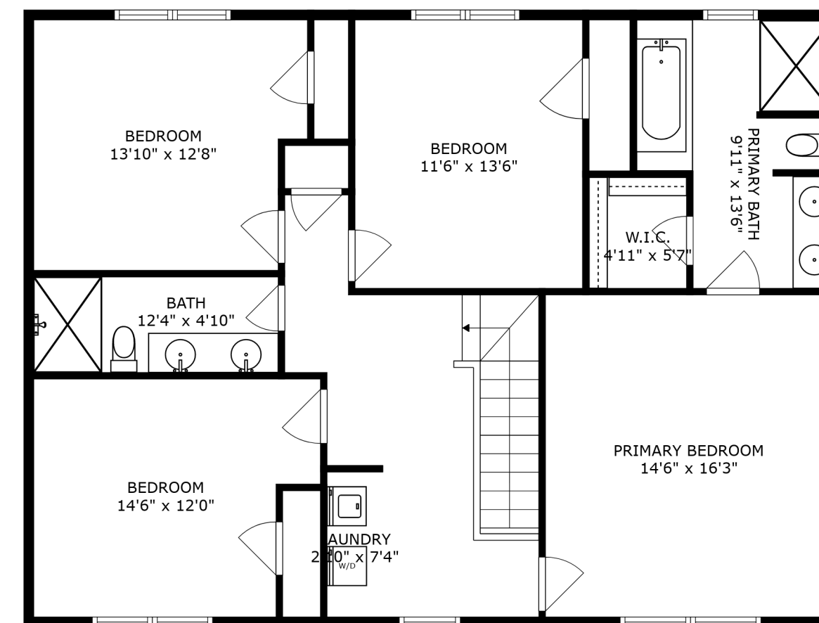
FLOOR 3
