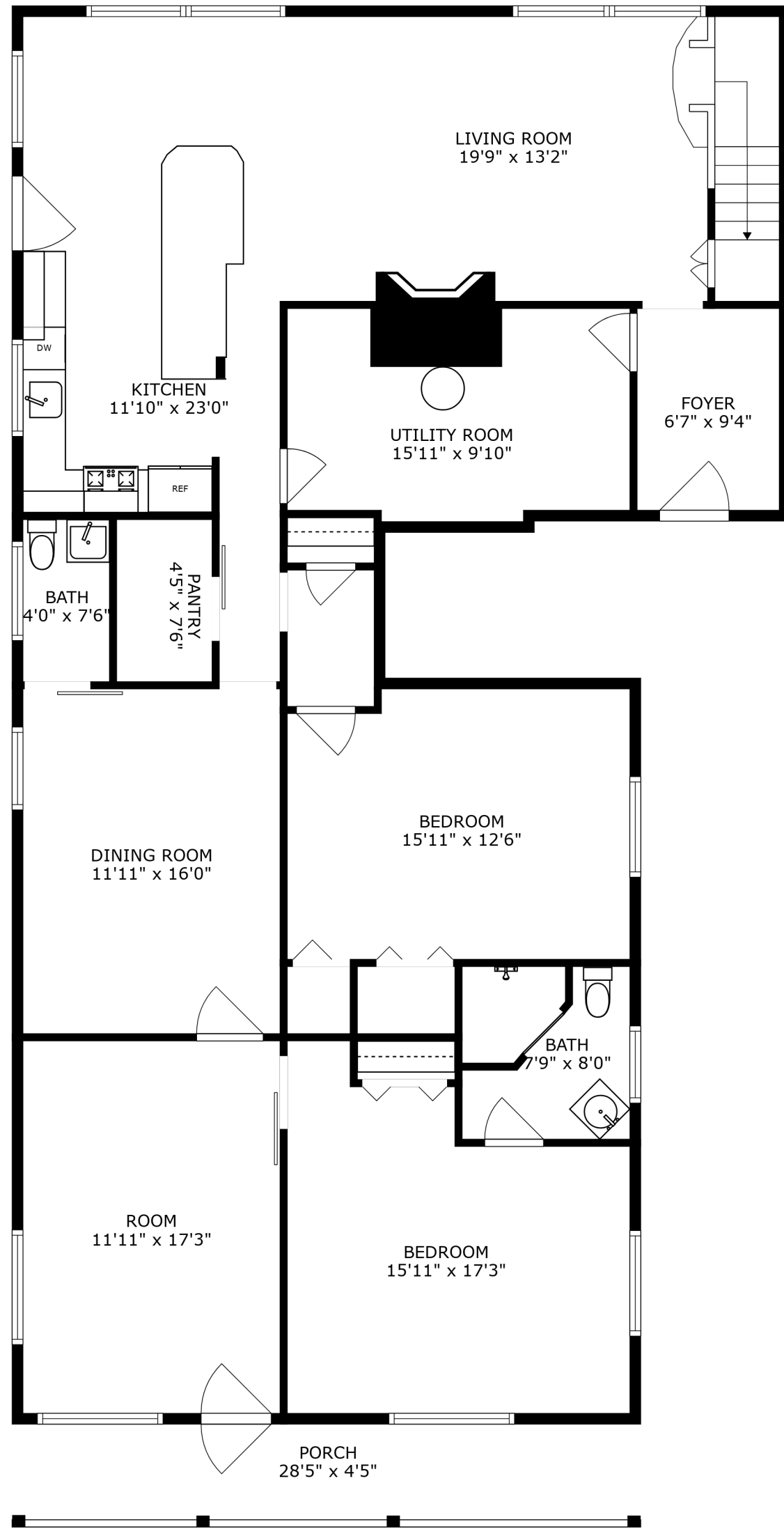
FLOOR 1
