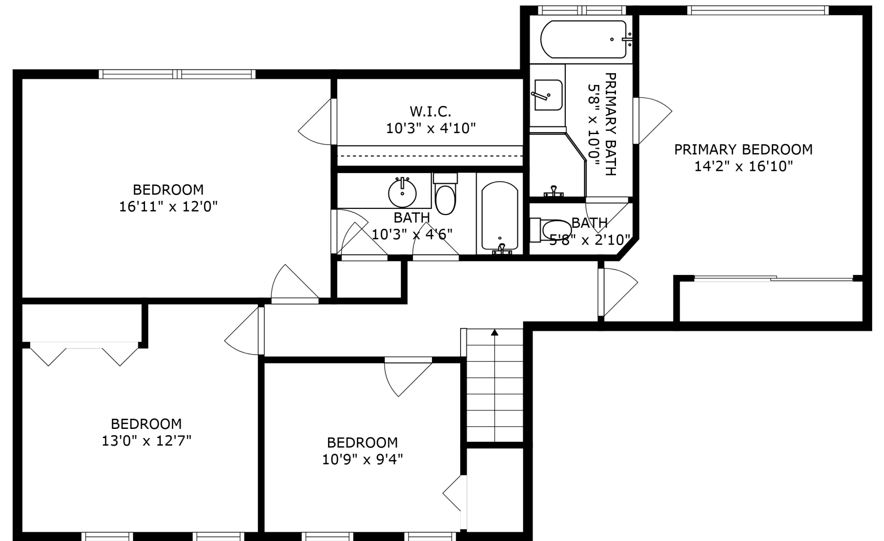
FLOOR 3
