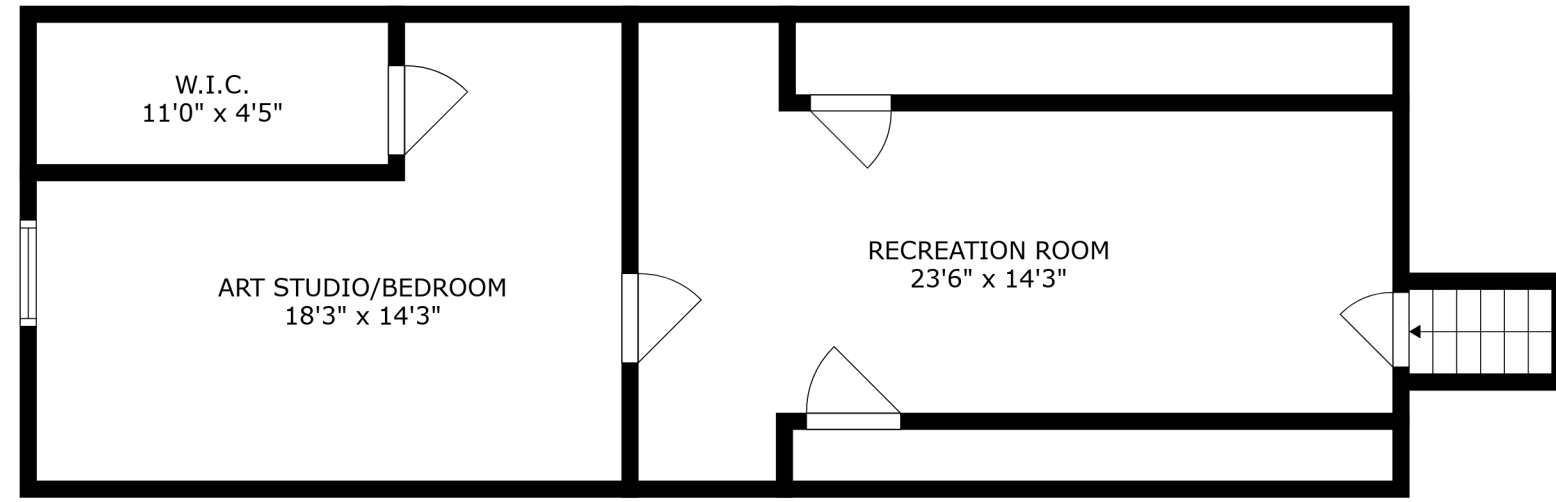
FLOOR 4
