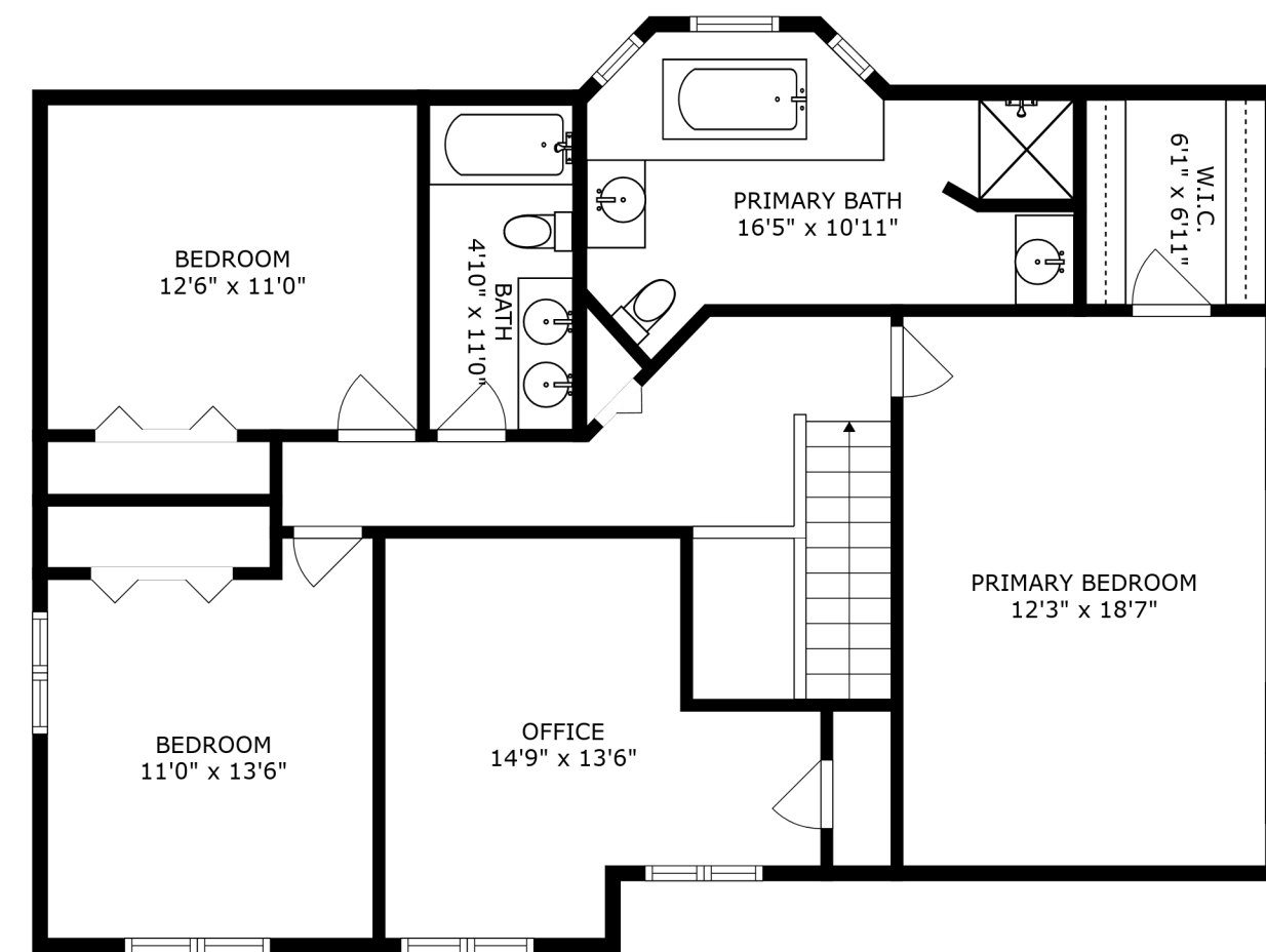
FLOOR 3
