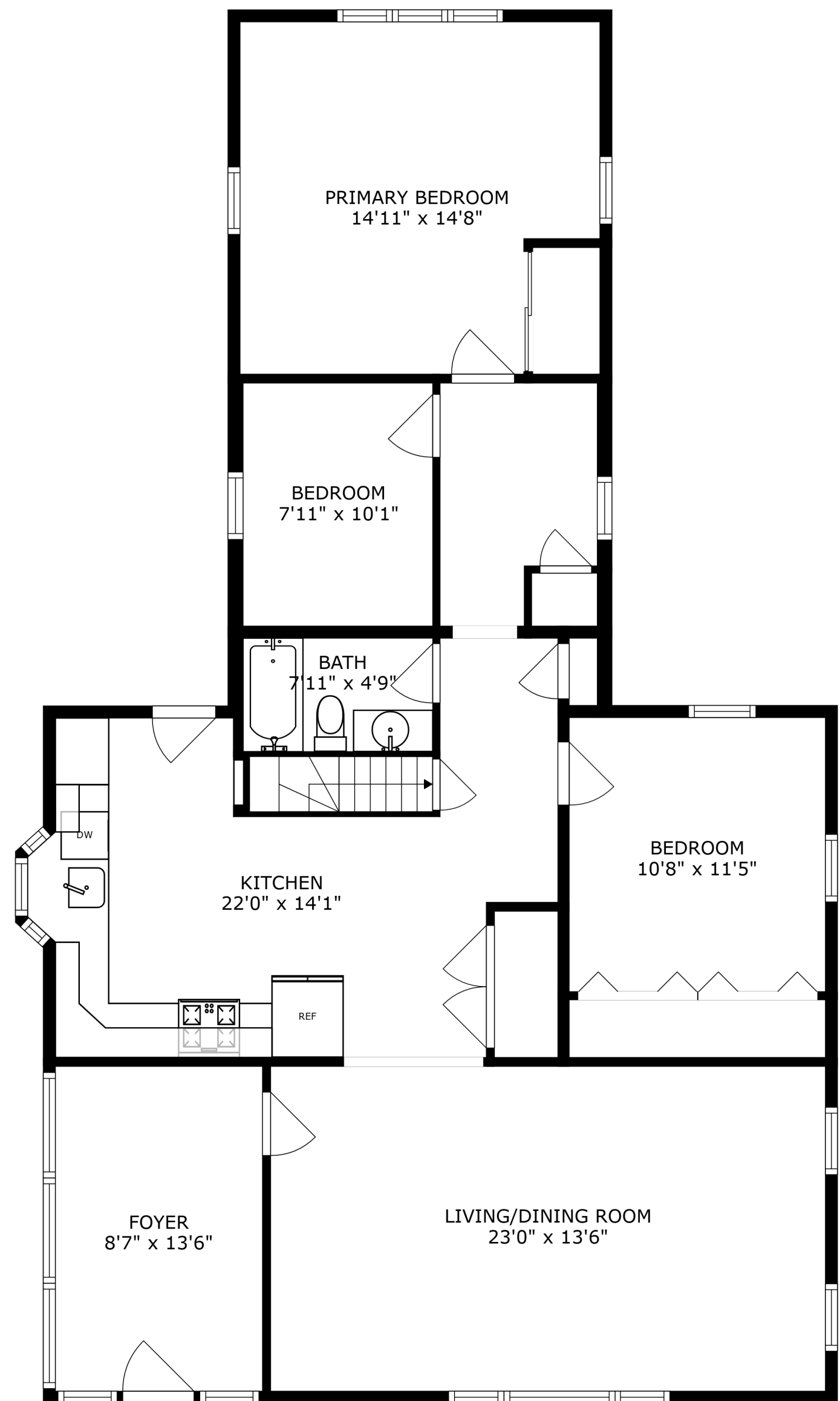
FLOOR 2
