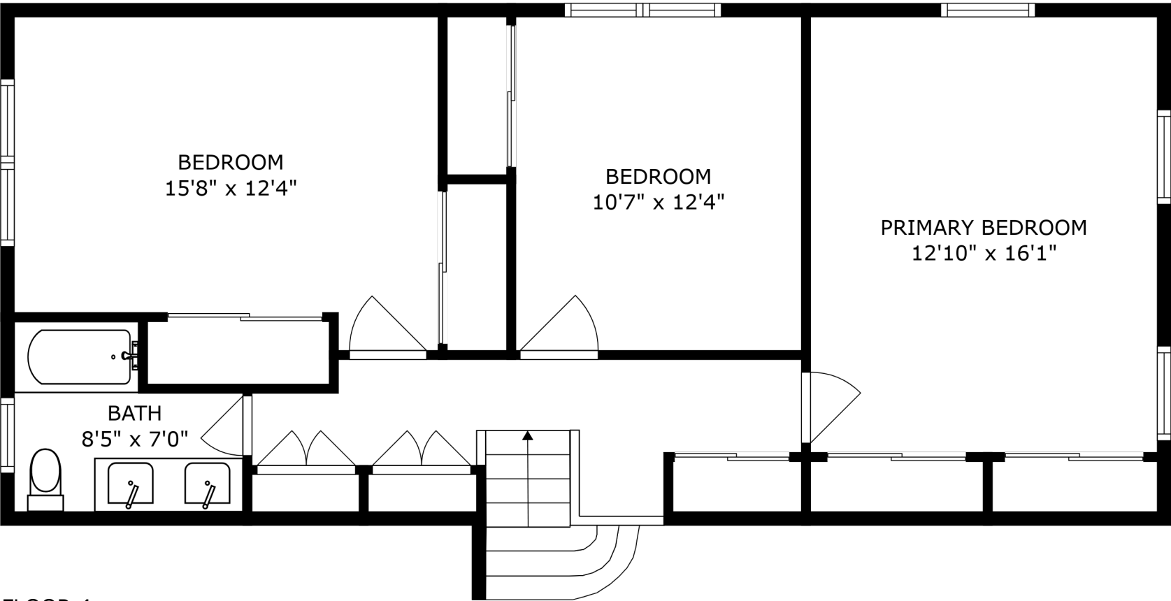
FLOOR 4
