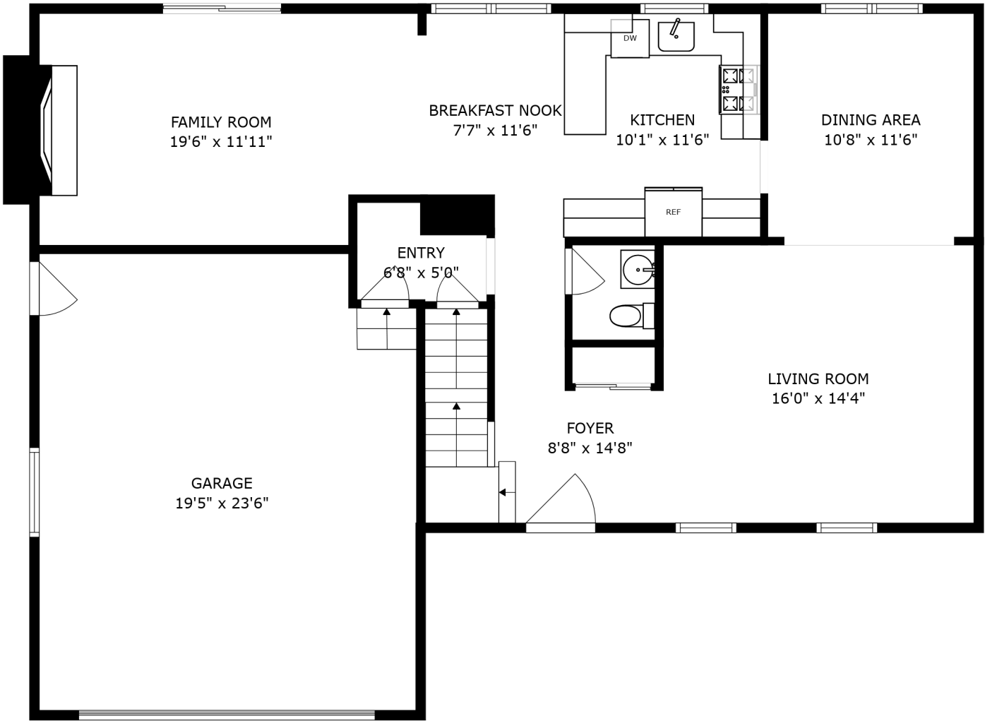
FLOOR 2
