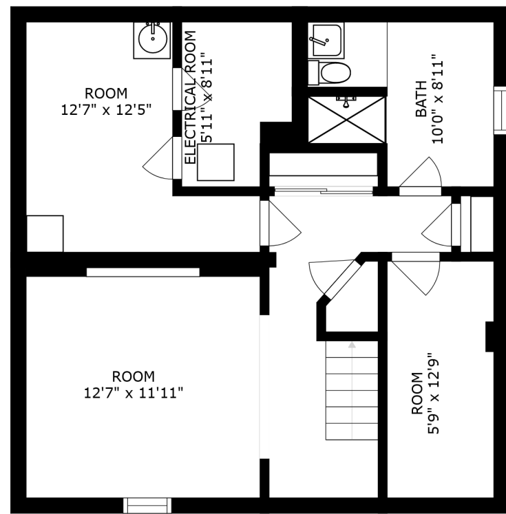
FLOOR 1
