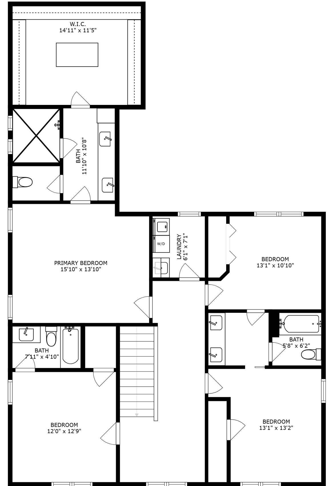
FLOOR 3
