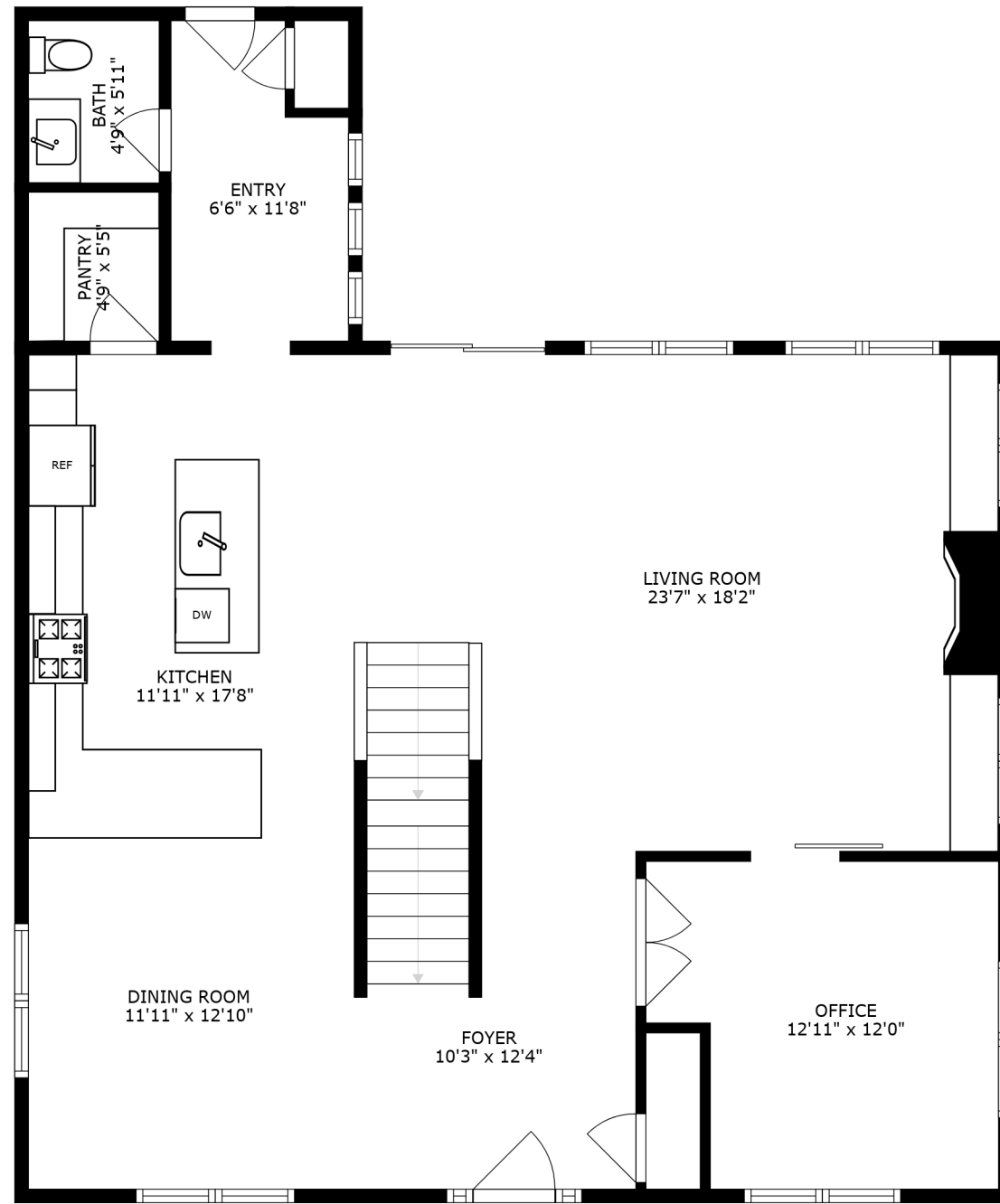
FLOOR 2
