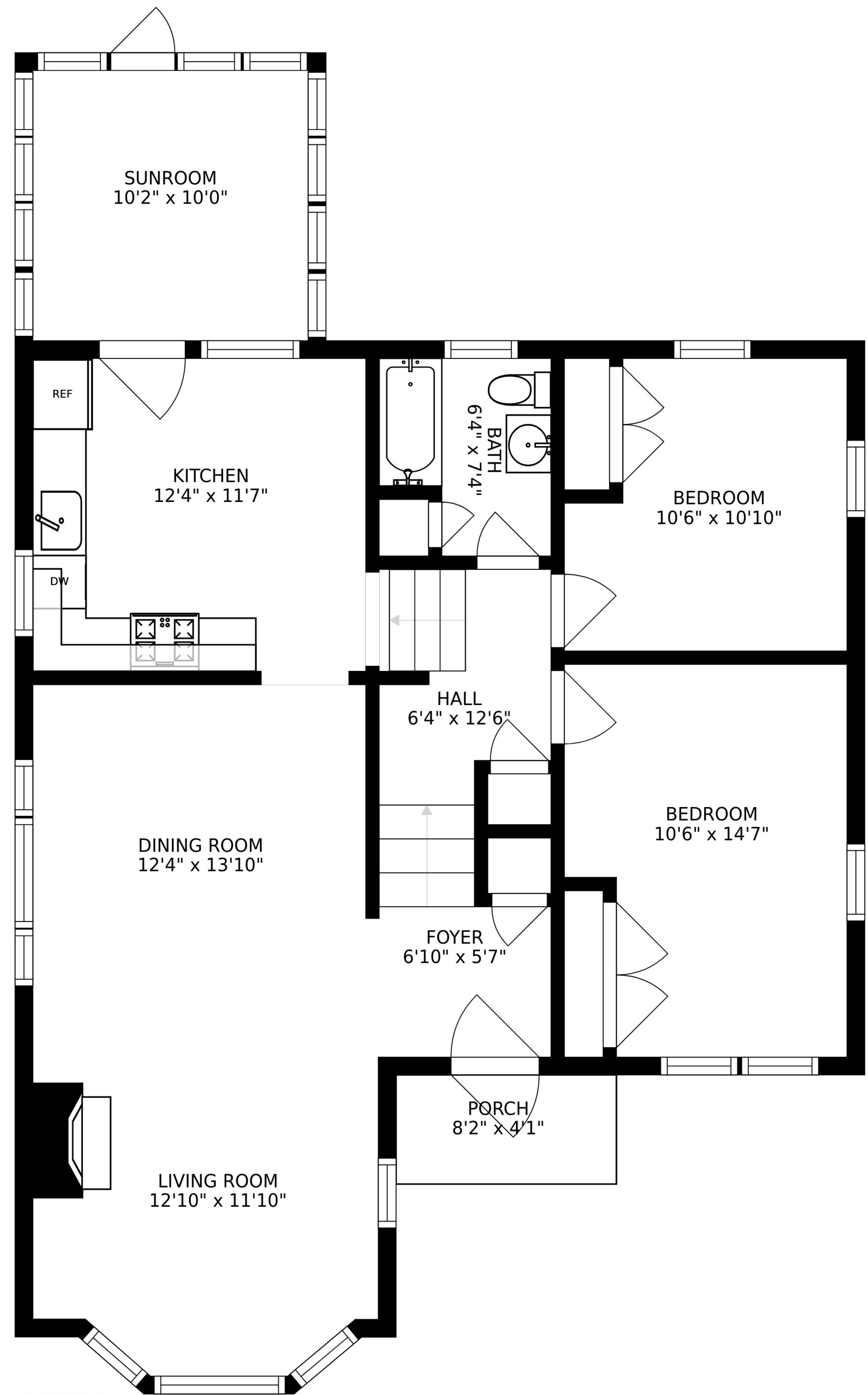
FLOOR 2
