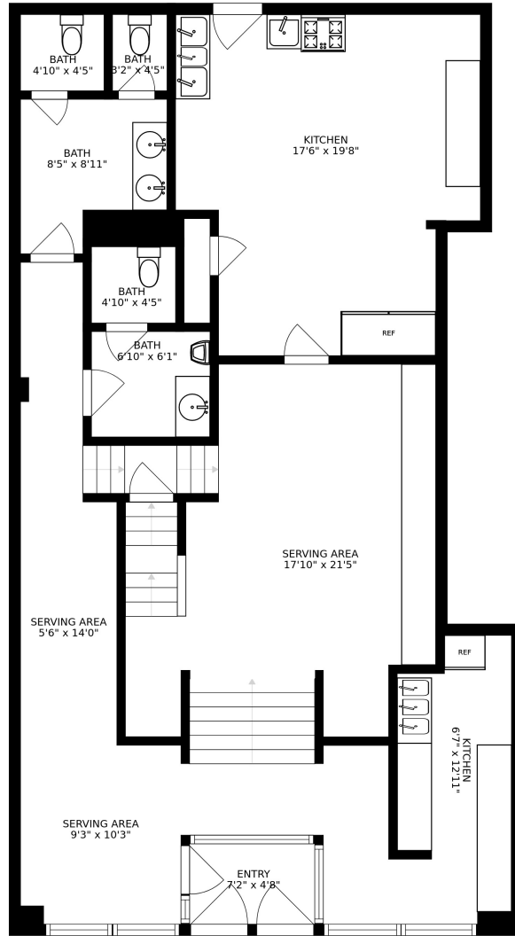
FLOOR 2
