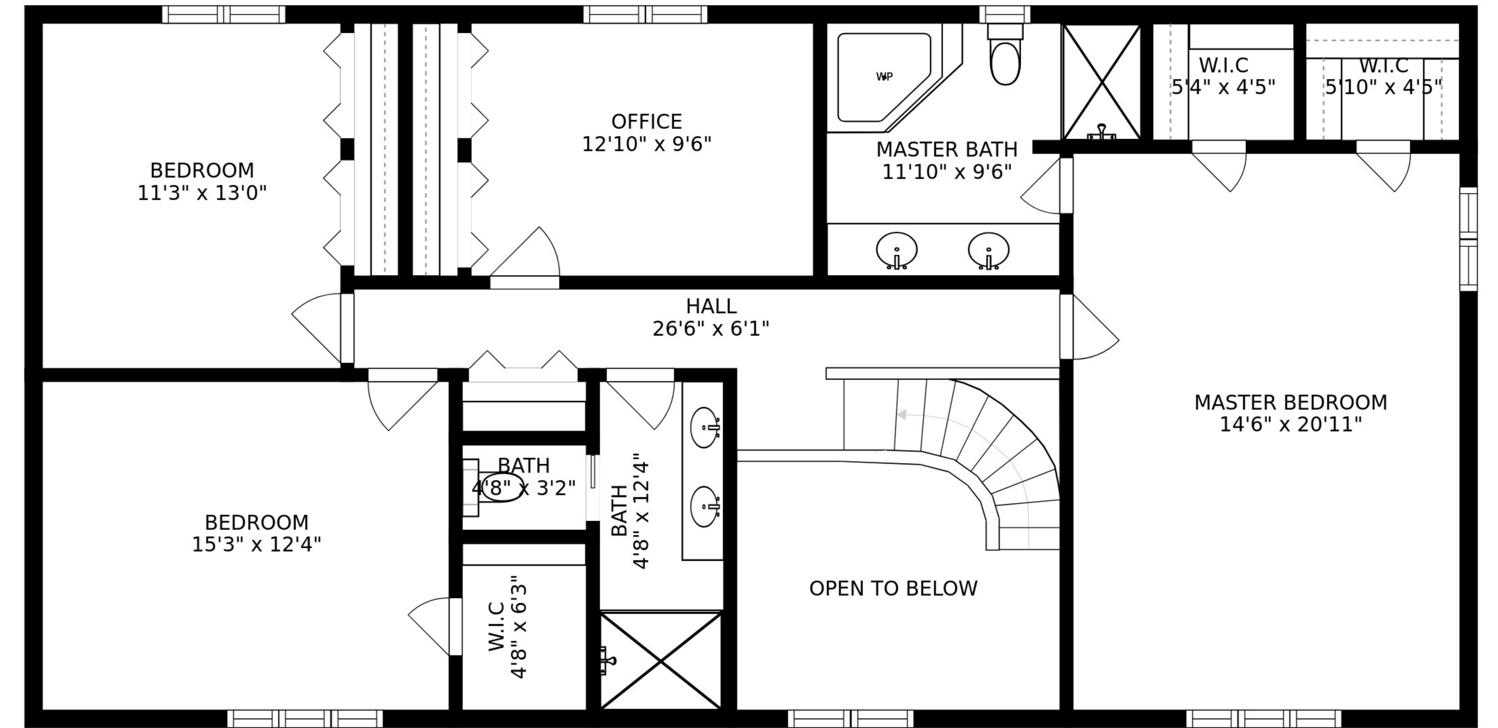
FLOOR 2
