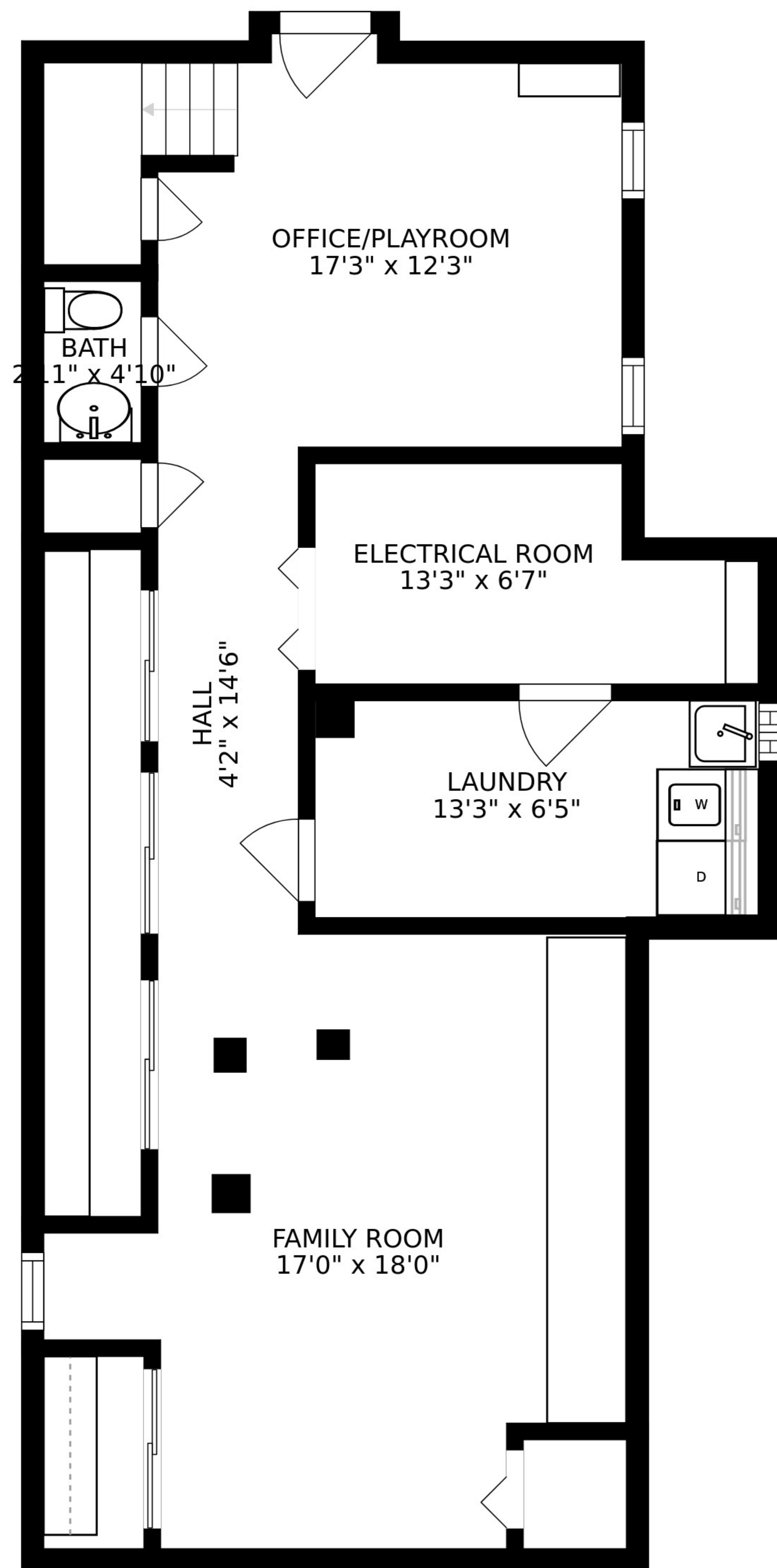
FLOOR 1
