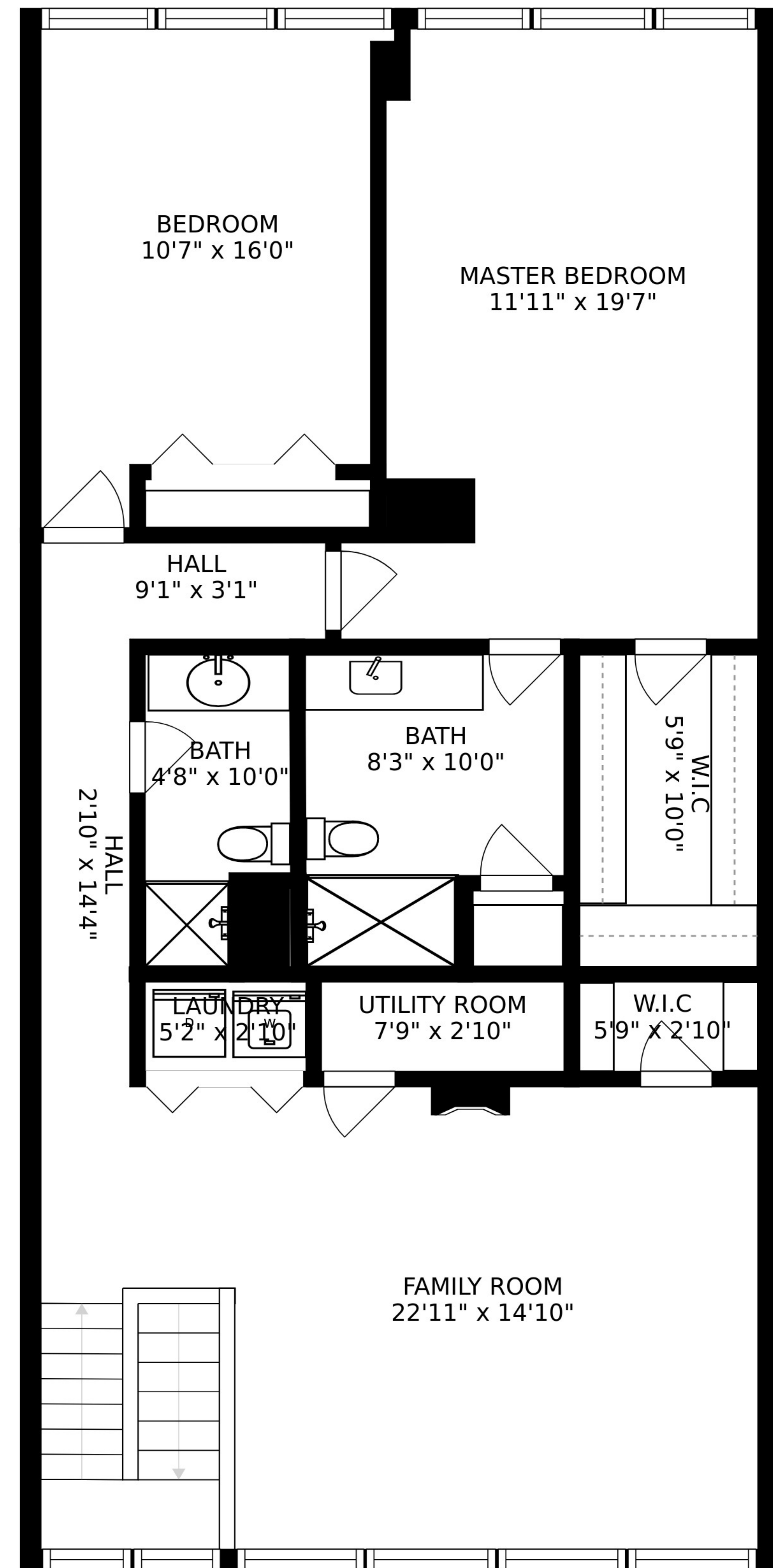
FLOOR 3
