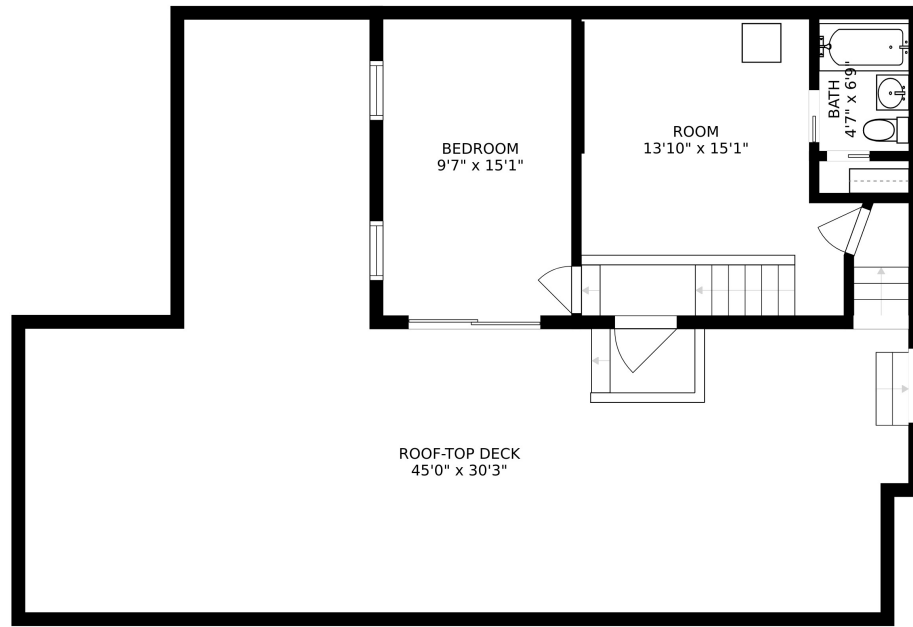
FLOOR 2
