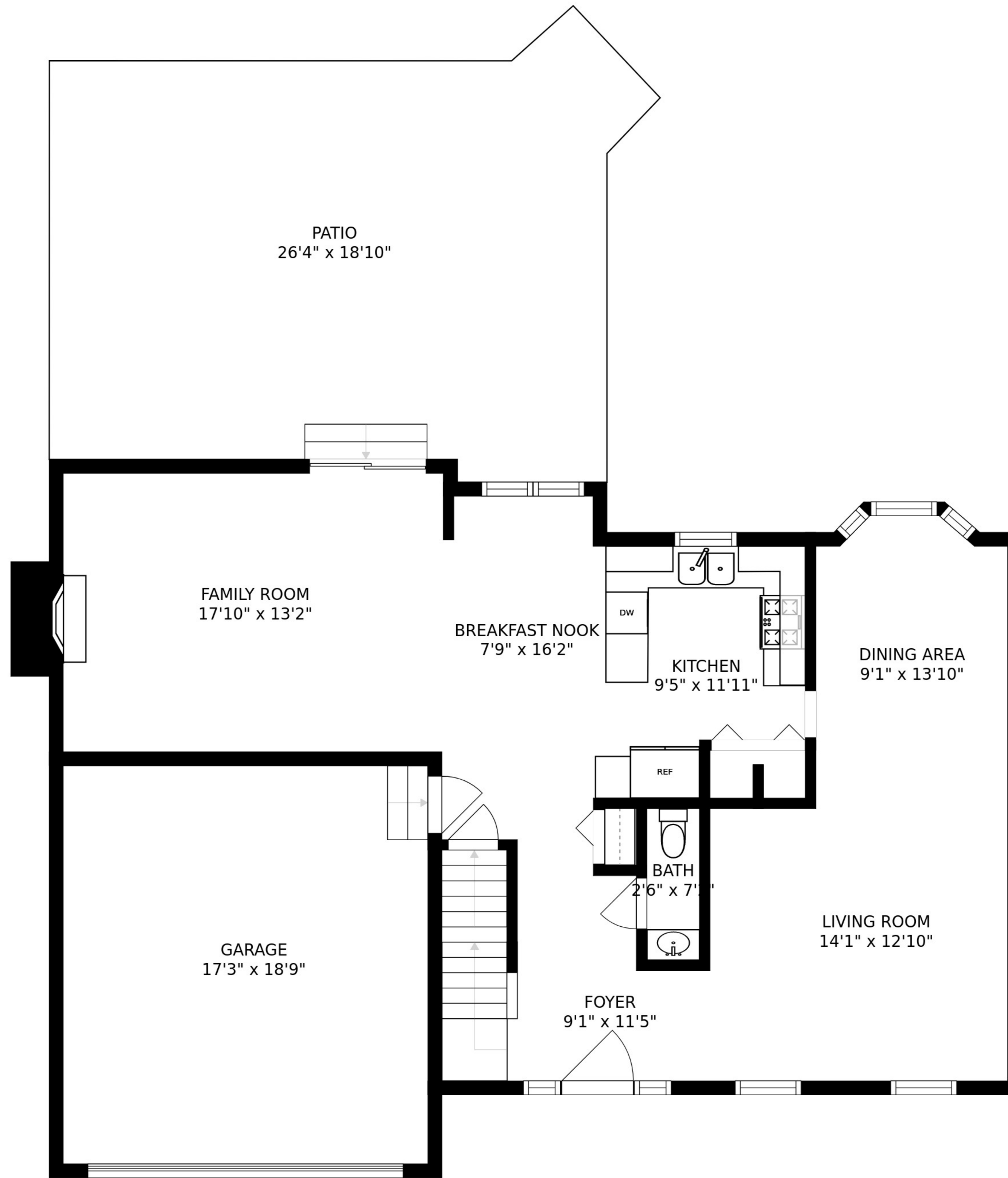
FLOOR 2
