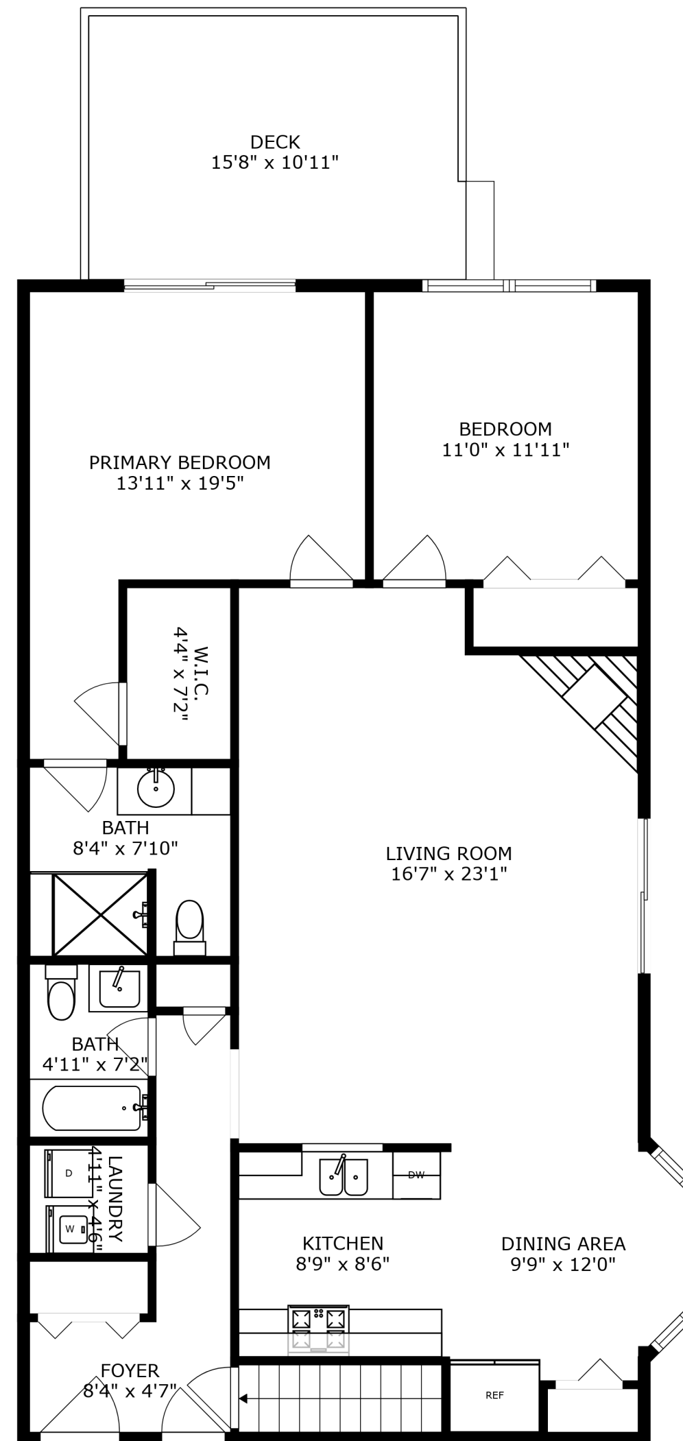
FLOOR 2
