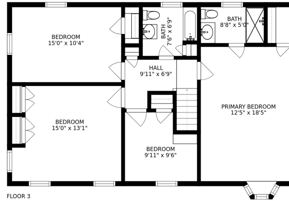
FLOOR 3
