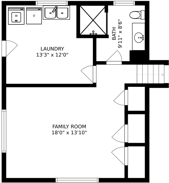
FLOOR 1
