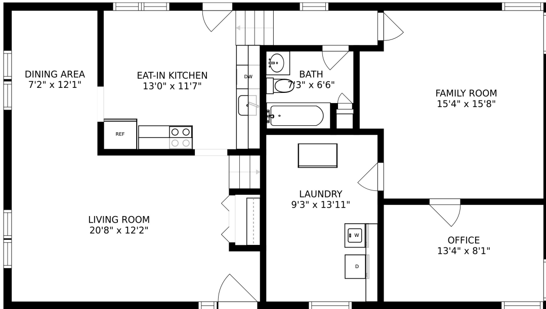
FLOOR 1
