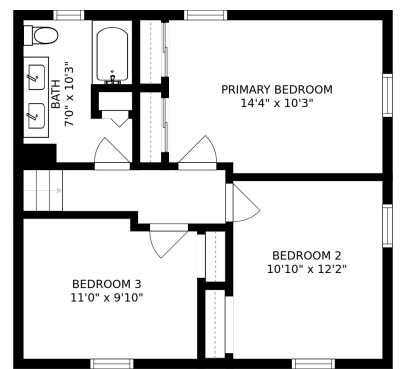
THIRD LEVEL
