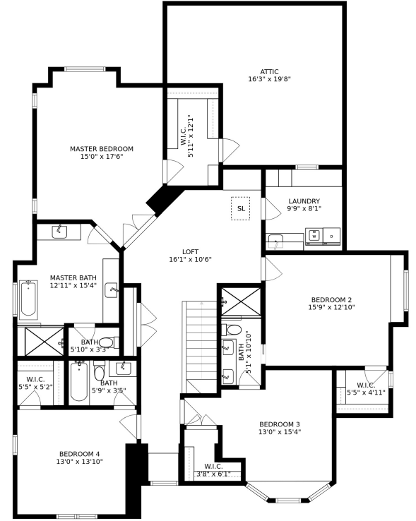
FLOOR 3
