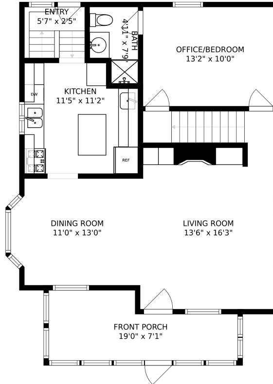
FLOOR 2
