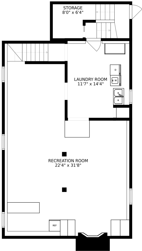
FLOOR 1
