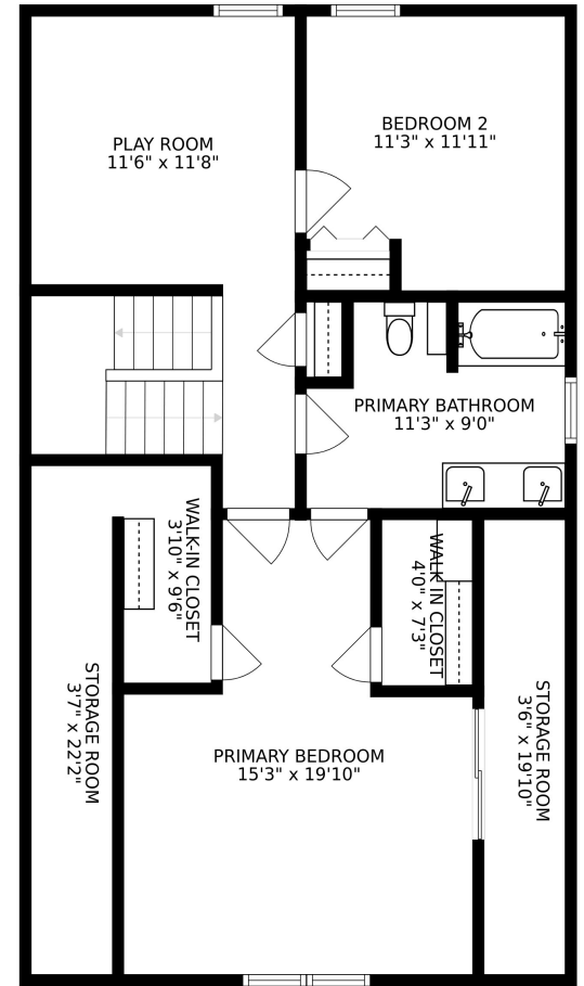
FLOOR 3
