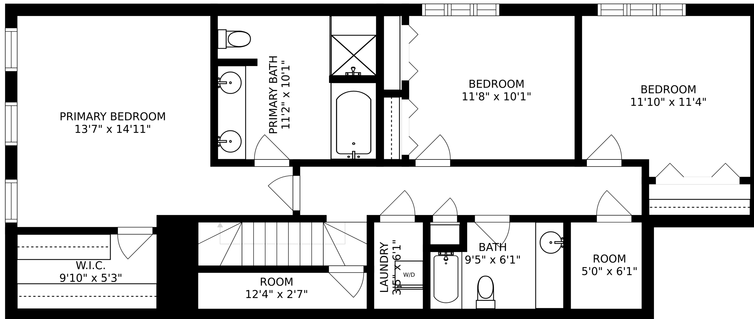
FLOOR 1
