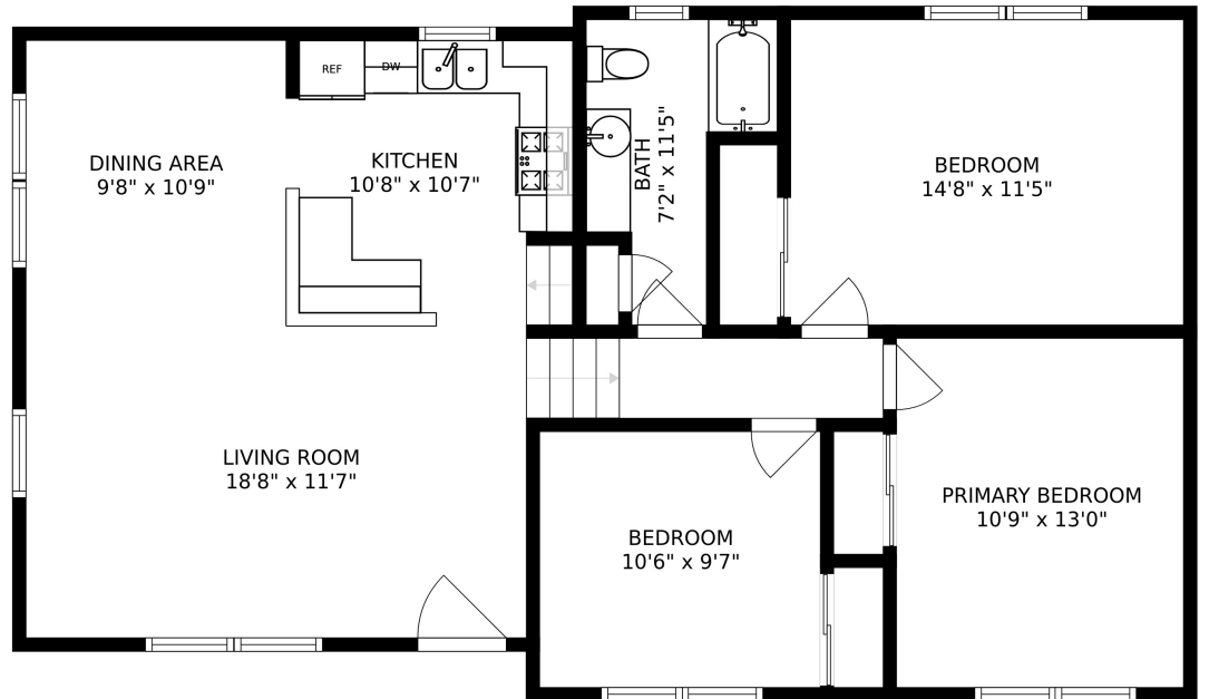
FLOOR 2
