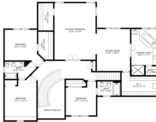
FLOOR 3
