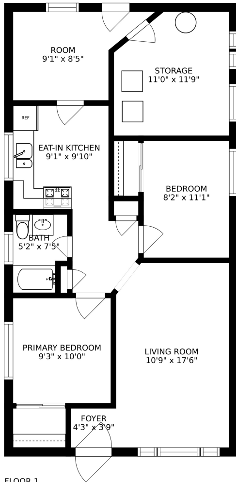
FLOOR 1
