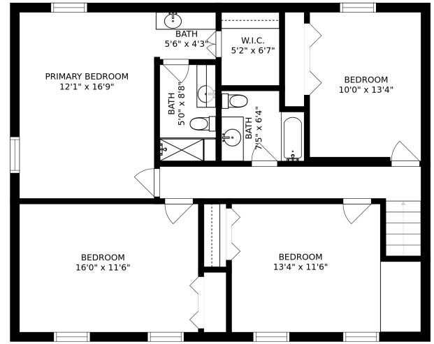
FLOOR 3
