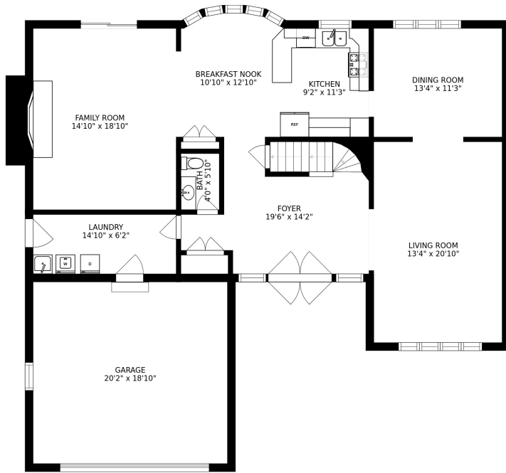
FLOOR 2
