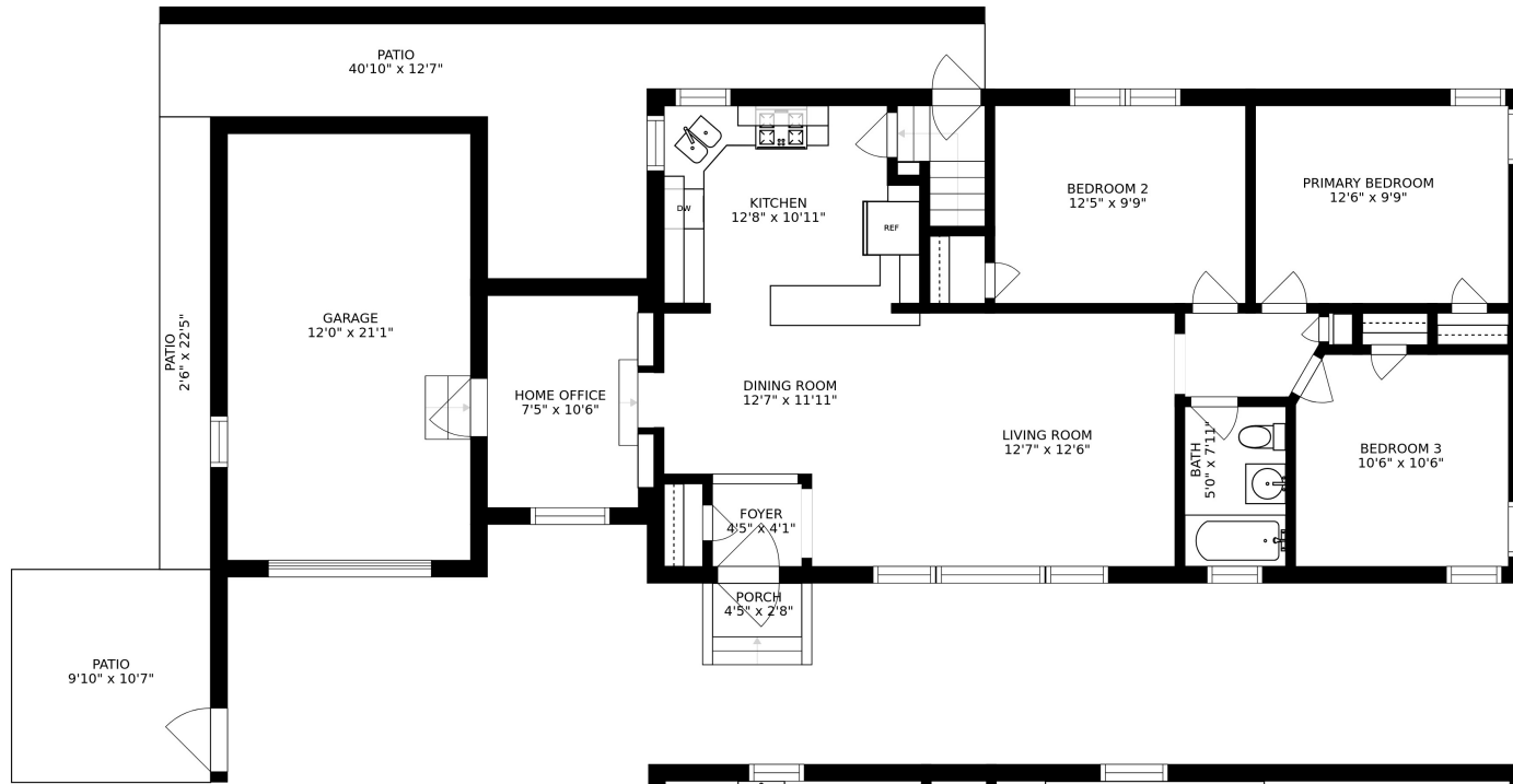
FLOOR 2
