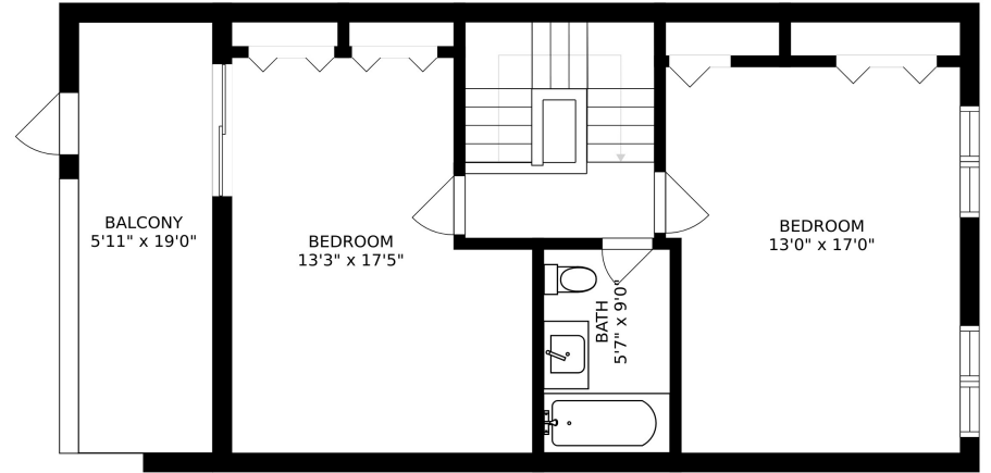
FLOOR 3
