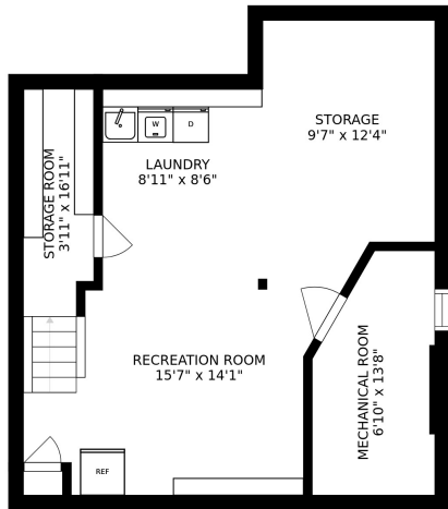
FLOOR 1
