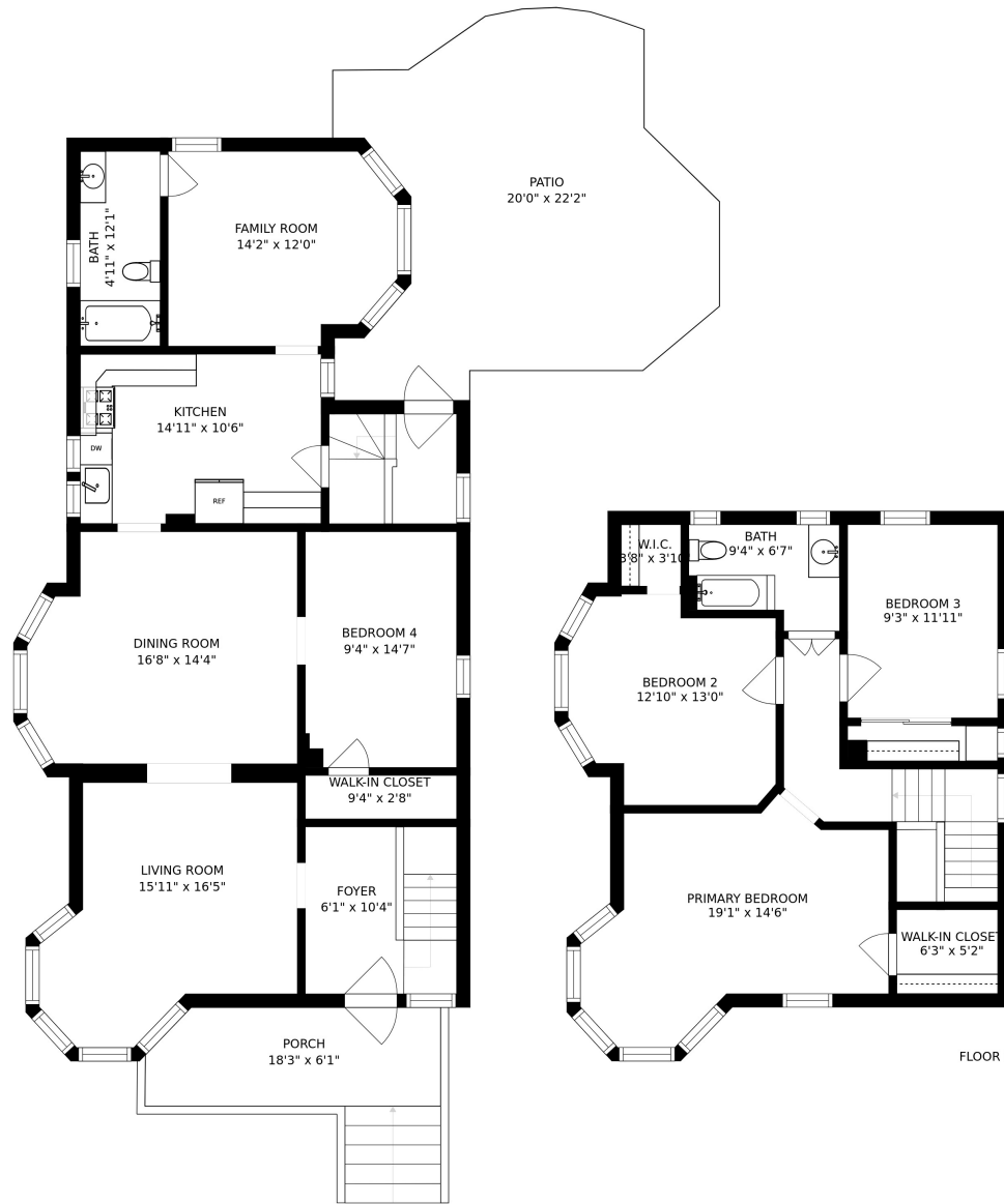
FLOOR 2
