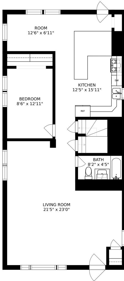
FLOOR 2
