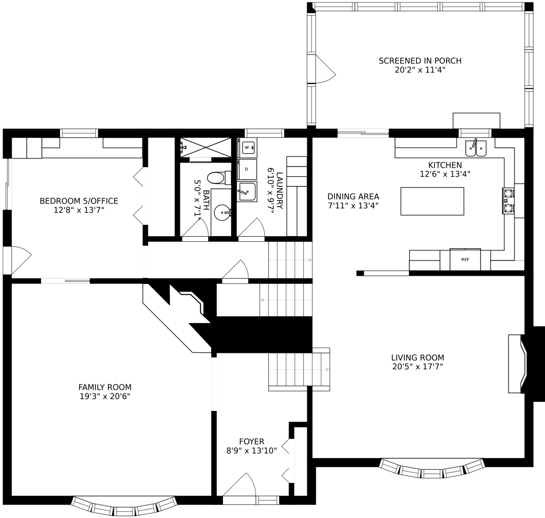
FLOOR 1
