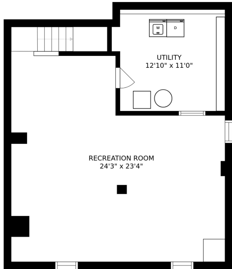
FLOOR 1
