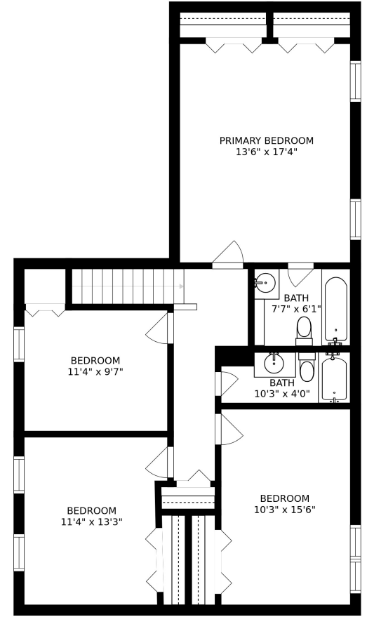
FLOOR 3
