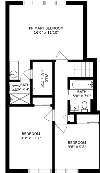
FLOOR 3
