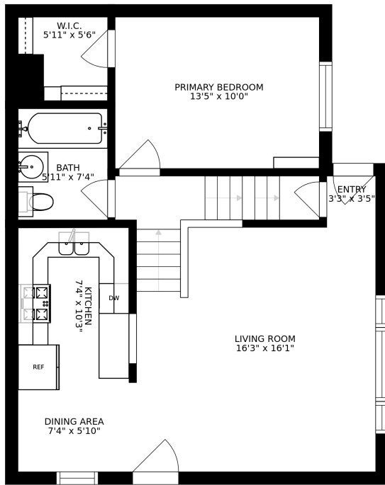
FLOOR 2
