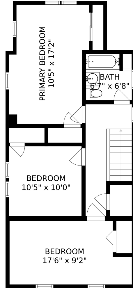
FLOOR 3
